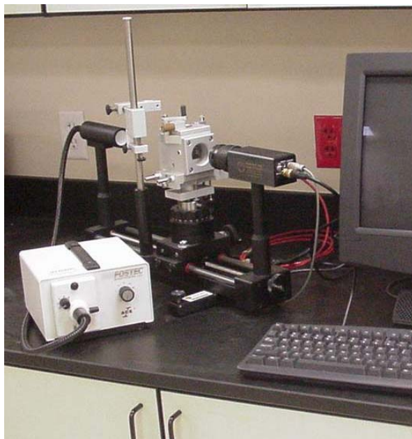
Rame-Hart 100, Goniometer (Membrane Contact Angle Measurement)
