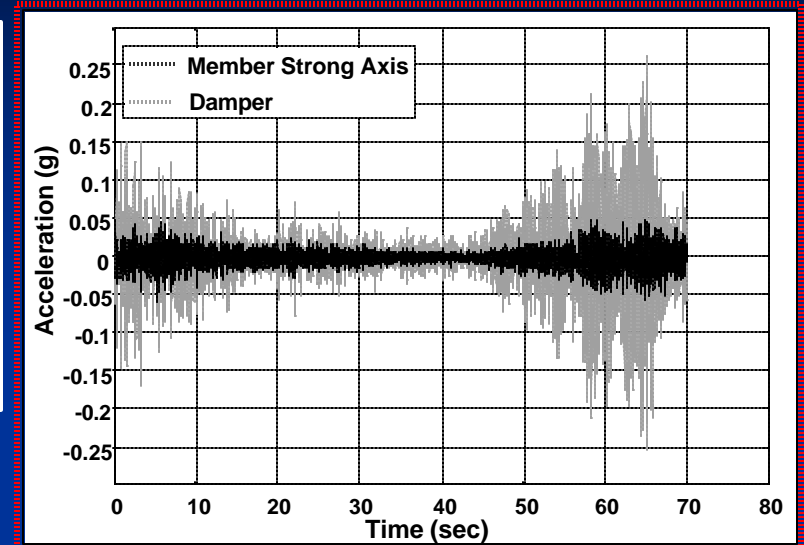
Accelerometers on absorbers
