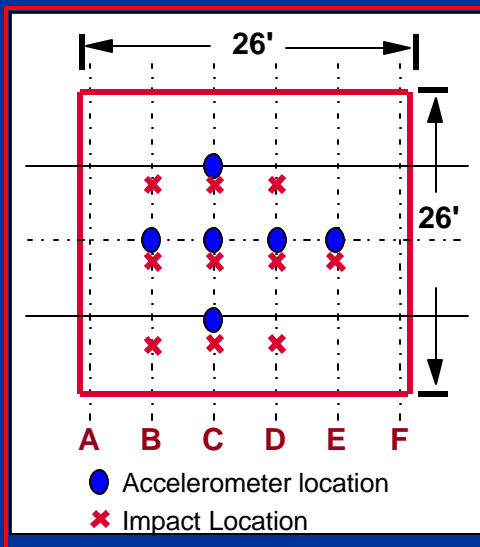
Impact Test Instrumentation
