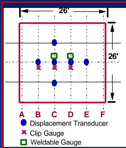
Load Test Instrumentation
